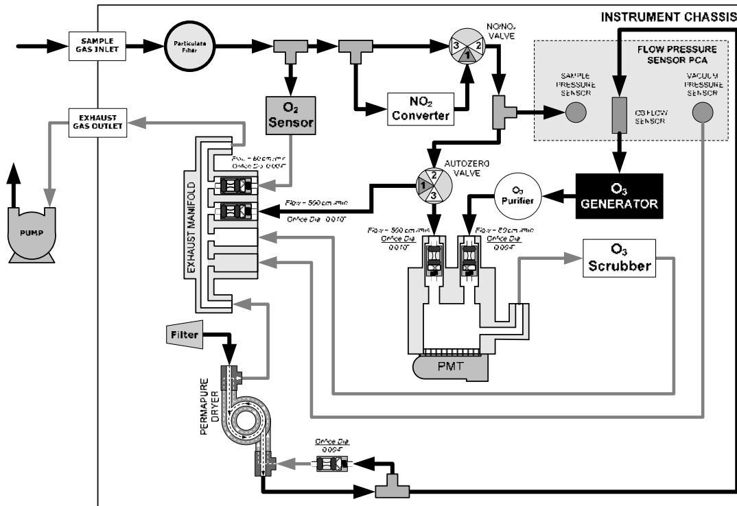
Figure 3-4: Base Configuration M200E Internal Pneumatics with O 2 Sensor Installed
