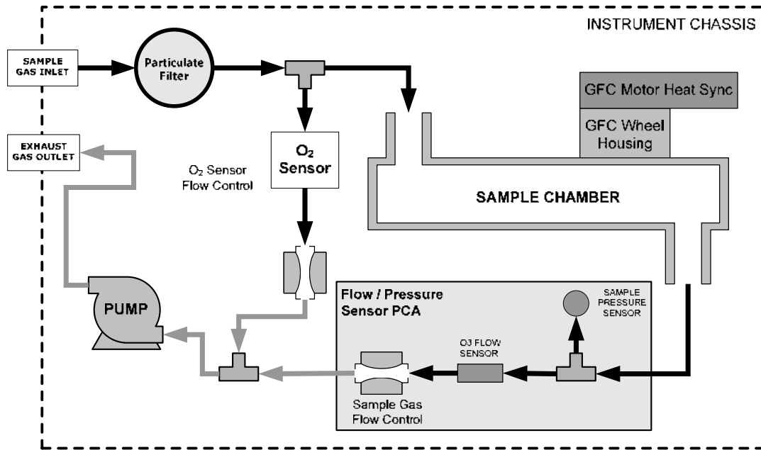
Figure 3-7: Base Configuration M300E Internal Pneumatics with O 2 Sensor Installed
