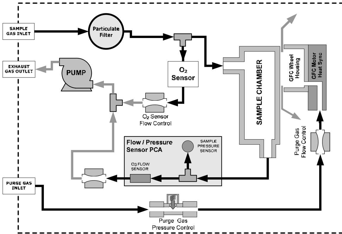
Figure 3-8: Base Configuration M360E Internal Pneumatics with O 2 Sensor Installed
