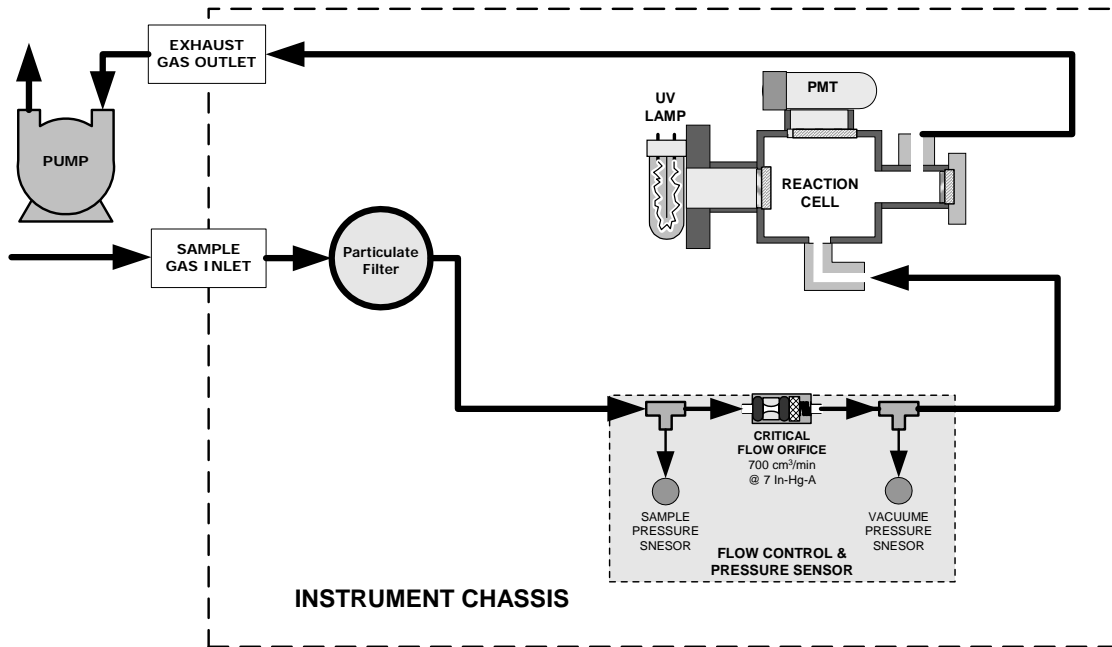
Figure 9-2: Pneumatic Diagram of the M100EH – Base Configuration
